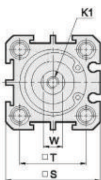
Bore \phi 20 - \phi 25
