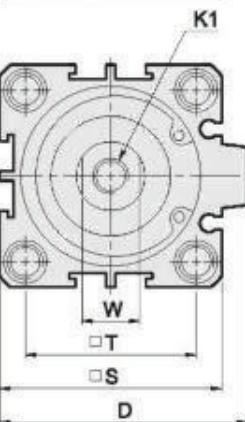
Bore \phi 32 - \phi 100
