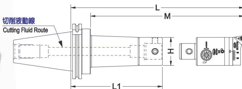
DIN69871A 搪孔刀柄 DIN69871A Taper Shank
